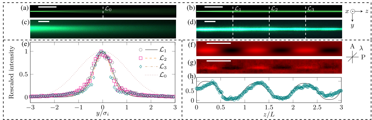
FIG. 2. Simulated (a),(b) ( x -averaged beam intensity) and experimental (c),(d) images (scattered laser light) of a beam propagating in a FLC sample in the linear (a),(c) and nonlinear (b),(d) optical regime. Simulated (f) and experimental (g) POM images, with the orientations of the polarizer, \lambda -wave plate and analyzer represented schematically on the right. The white bars represent 100 \mu\text{m} in (a)–(d) and the half-periodicity L/2 of the POM signal in (f),(g) [43 \mu\text{m} for (f), 143 \mu\text{m} for (g)]. The axes orientation on the right applies to (a)–(g). (e) Experimental (marks) and simulated (lines) rescaled intensity profiles along the lines \mathcal{L}_{1,2,3} defined in (b),(d). \sigma_i is the input beam waist. For comparison, the profile \mathcal{L}_0 of the diffracting beam presented in (a) is also shown. (h) Experimental (marks) and simulated (line) rescaled 1D profile of POM images (f),(g) along the beam axis.
