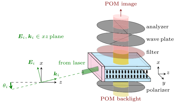
FIG. 1. Schematic of the experimental setup. The CLC layer is sandwiched between two plates treated for homeotropic boundary conditions, and the laser beam is injected from the side through a cover slip (in pink) also treated for vertical alignment of the CLC molecules. For sufficiently thin samples, the equilibrium bulk orientation of the CLC molecules is the unwound state \mathbf{n}_0 parallel to x .
