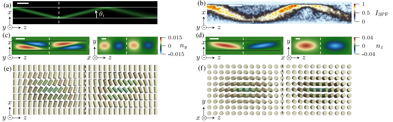
FIG. 3. xz slice of the simulated beam intensity (a) and experimental tomography signal I_{3PF} (b). (c) Color-coded slices of n_y ( y component of the director field) in the xz and yz planes. (d) Same as (c) with n_z . (e),(f) Schematic representation of the reorientation of the director (depicted with cylinders) in the xz and yz planes. The reorientation angle was greatly exaggerated and the \{x, y\} directions were magnified for clarity. The white bars represent 10 \mu\text{m} . The dashed lines represent the same z .
