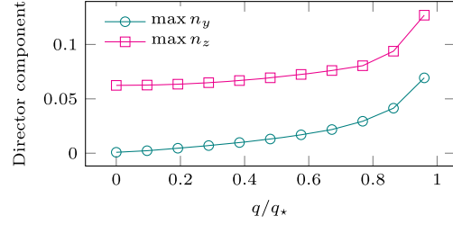
FIG. 4. Maxima of n_y and n_z plotted as a function of q/q_* , assuming that all other simulation parameters (beam power, insertion angle, sample thickness) stay constant.
