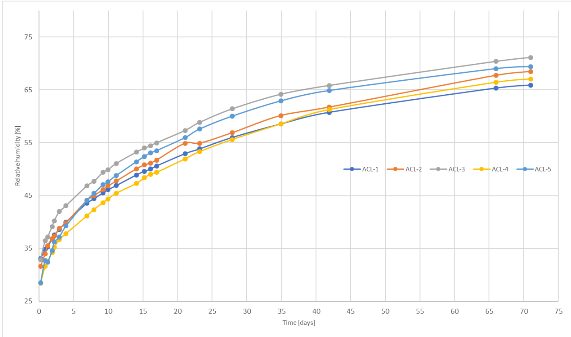
Attachment Figure 5: ACL in 30°C/75% RH
