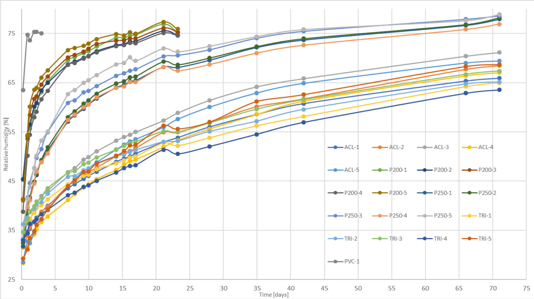
Attachment Figure 1: All configurations in 30°C/75% RH
