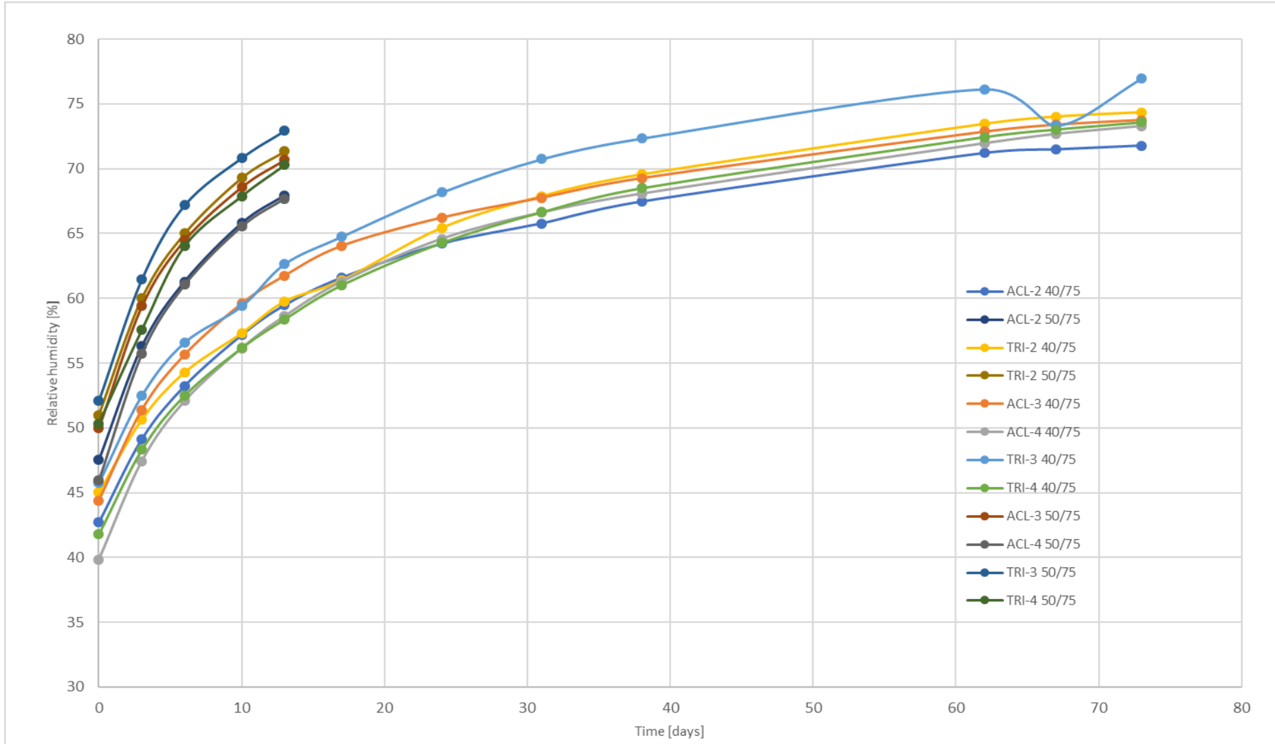
Attachment Figure 8: Comparison of 40°C/75% RH and 50°C/75%RH
