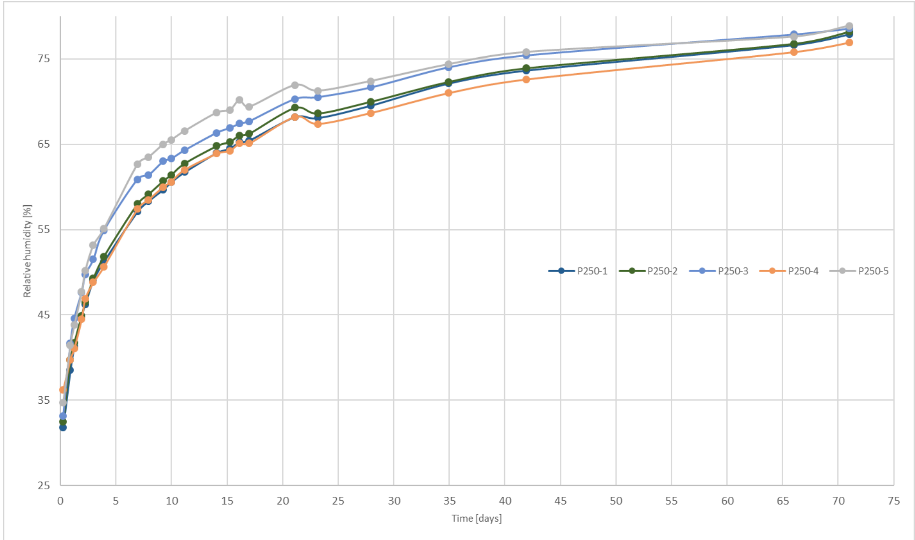
Attachment Figure 3: P250 in 30°C/75% RH
