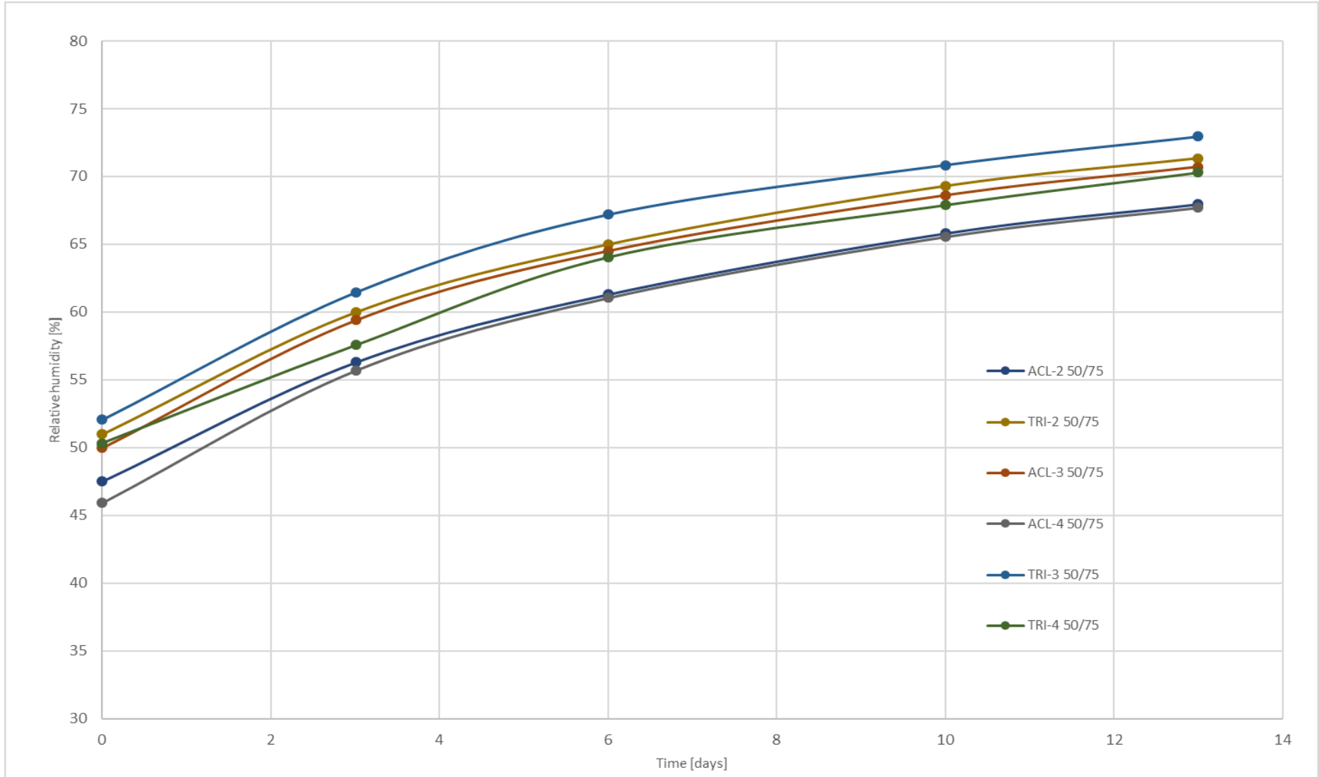
Attachment Figure 7: All 40°C/75% RH conditions configurations
