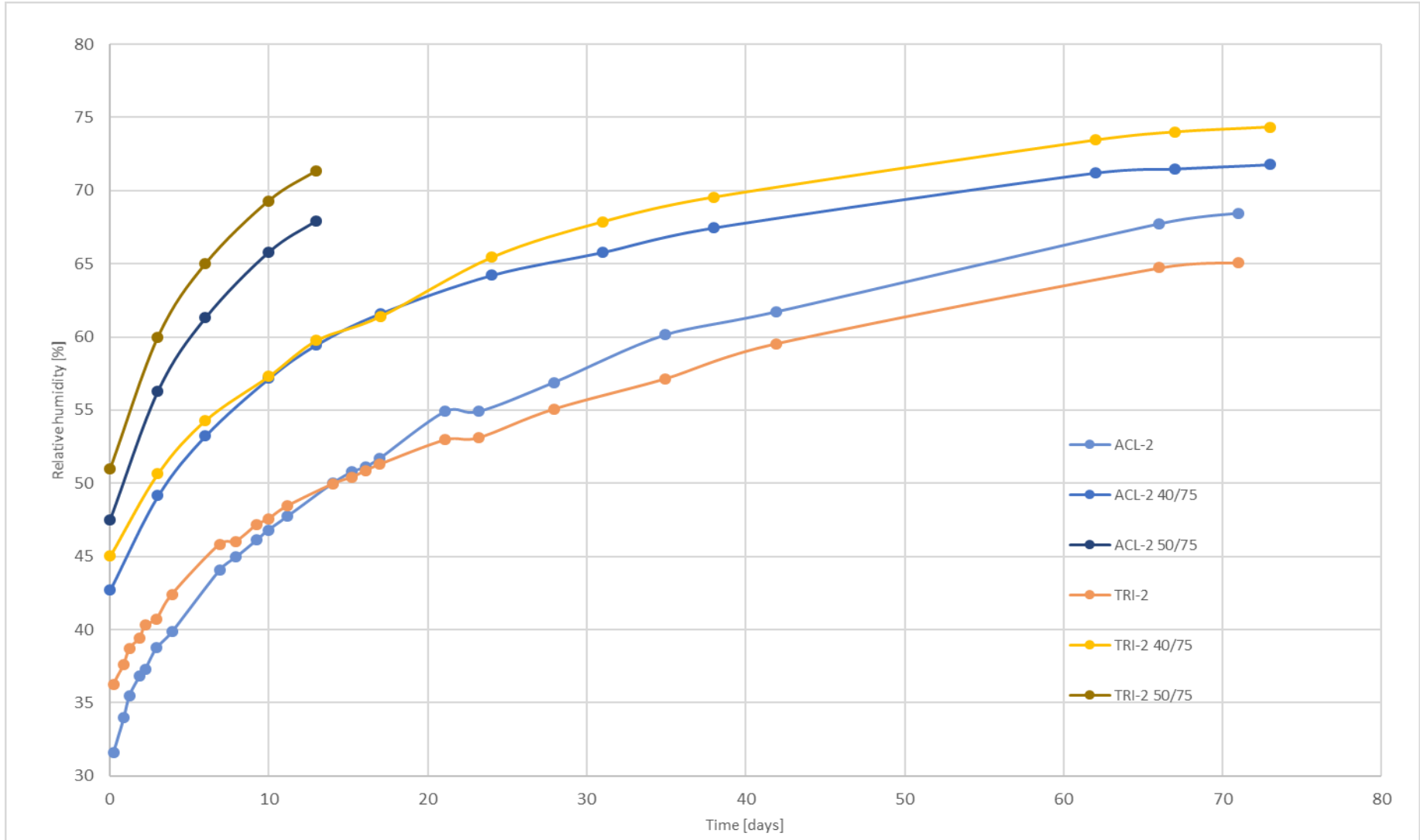
Attachment Figure 9: Comparison of ACL and TRI in all three conditions
