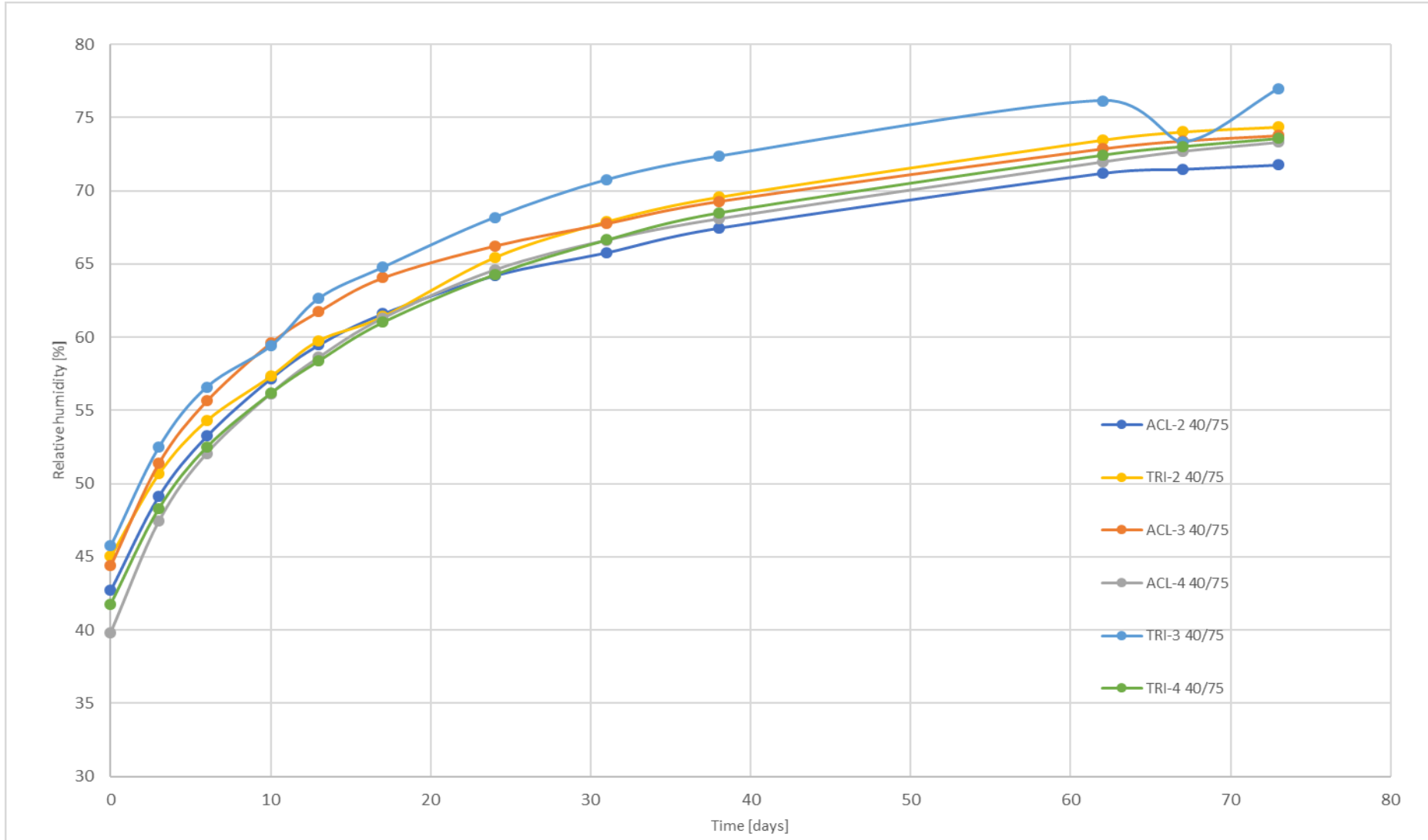
Attachment Figure 6: All 40°C/75% RH conditions configurations
