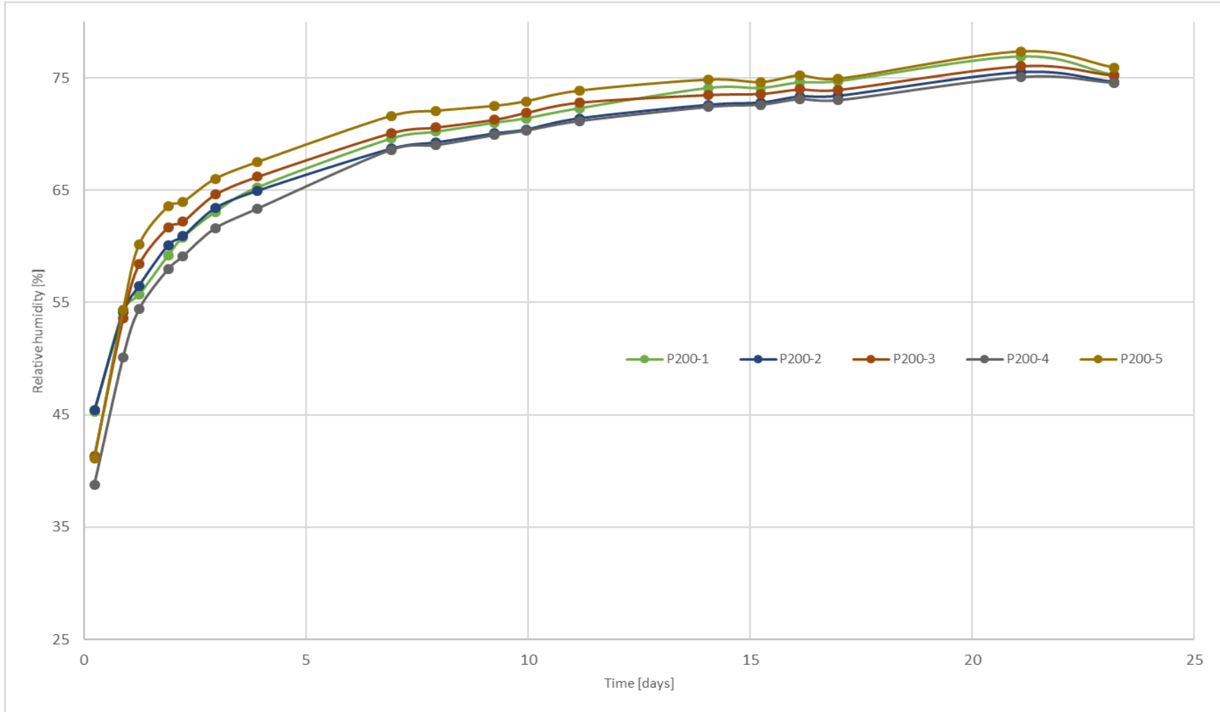
Attachment Figure 2: P200 in 30°C/75% RH
